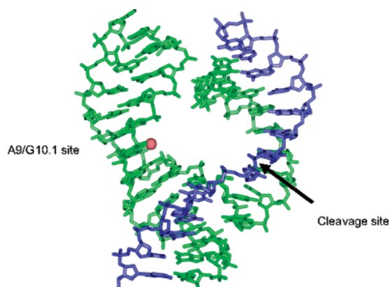
Figure 2. Crystal structure of Hammerhead ribozyme (PDB 1HMH, ref 14) with a \text{Mn}^{2+} ion (red sphere) placed at the A9/G10.1 site.
