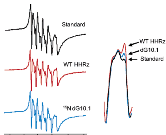
Figure 3. X-band EPR spectra of \text{Mn}^{2+} bound to hammerhead ribozymes. Inset shows an overlay of the sixth (highest-field) line of the EPR spectra of \text{Mn}^{2+} bound to WT HHRz, HHRz with a dG10.1 substitution, and \text{Mn}^{2+} in a buffer solution (Standard). Spectra were obtained at 10 K, with 250–350 \mu\text{M} HHRz samples in 1 M NaCl, 5 mM TEA, pH = 7.8, and 20% ethylene glycol. EPR instrument conditions were X-band (9.4 GHz), 0.2 mW microwave power, 100 kHz magnetic field modulation at an amplitude of 15 G.
