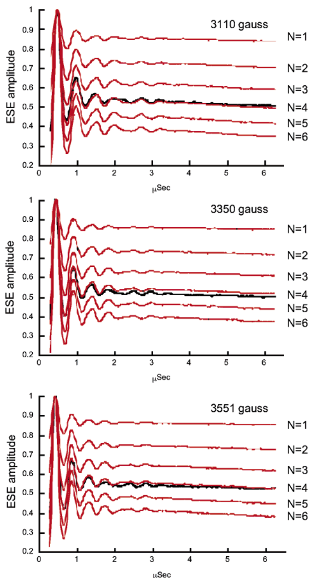
Figure 5. Hydration level of the high-affinity \text{Mn}^{2+} site in the hammerhead ribozyme determined by ^2\text{H} ESEEM spectroscopy. ^2\text{H} three-pulse ESE time-domain traces from deuterium-exchanged HHRz samples, ratioed by data obtained on natural-abundance HHRz samples (see Materials and Methods), are compared with data calculated for hydration levels of N = 1-6 ^2\text{H}_2\text{O} \text{Mn}^{2+} ligands. Data are plotted as a function of T ( \mu\text{s} ) (see Materials and Methods) and were obtained at three different magnetic field values with \eta values (in parentheses) selected for suppression of proton modulation: 3110 G (228 ns); 3350 G (210 ns); 3551 G (198 ns). The average fit to these data gives a value of 4.08 \pm 0.12 \text{H}_2\text{O} molecules coordinated to the HHRz-bound \text{Mn}^{2+} ion.
