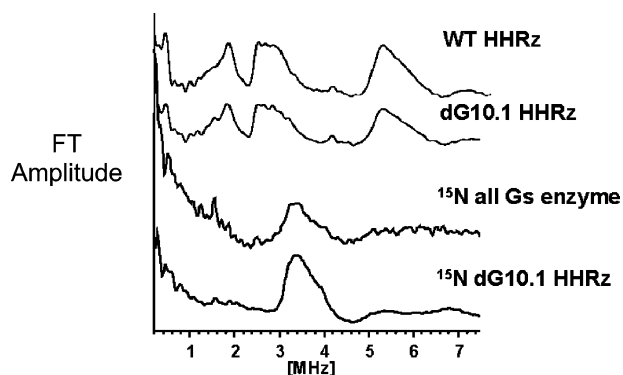
Figure 4. ^{14/15}\text{N} three-pulse ESEEM spectra of \text{Mn}^{2+} bound to the hammerhead ribozyme. Wild type and dG10.1 HHRz show similar ^{14}\text{N} ( I = 1 ) ESEEM Fourier transform traces, consistent with \text{Mn} –guanine coordination. The “ ^{15}\text{N} all G’s enzyme” HHRz, in which all guanines on the enzyme strand are labeled with ^{15}\text{N} , shows an ESEEM pattern consistent with \text{Mn} – ^{15}\text{N} ( I = 1/2 ) coordination. 22 A nearly identical spectrum is observed with specific ^{15}\text{N} labeling of G10.1, identifying G10.1 as the \text{Mn}^{2+} ligand. Experiment conditions: magnetic field strength 3600 G, \tau = 192 ns, \eta/2 pulse length 15 ns, microwave power 3.2 W.
